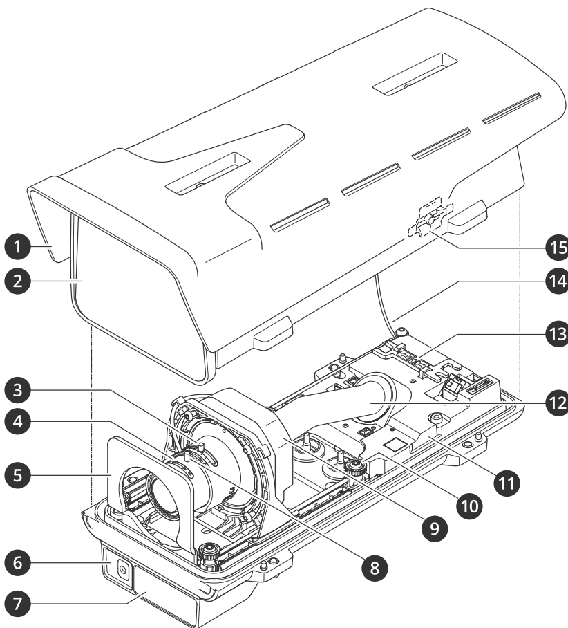
AXIS P1388-LE Box Camera
