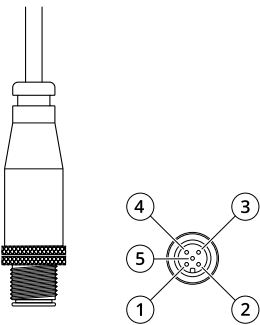
5-pin DC connector
