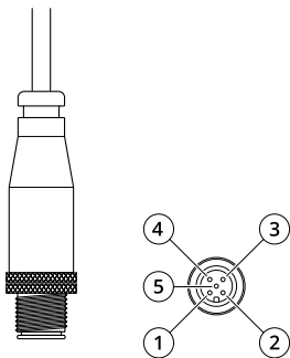
Conector CC com 5 pinos
