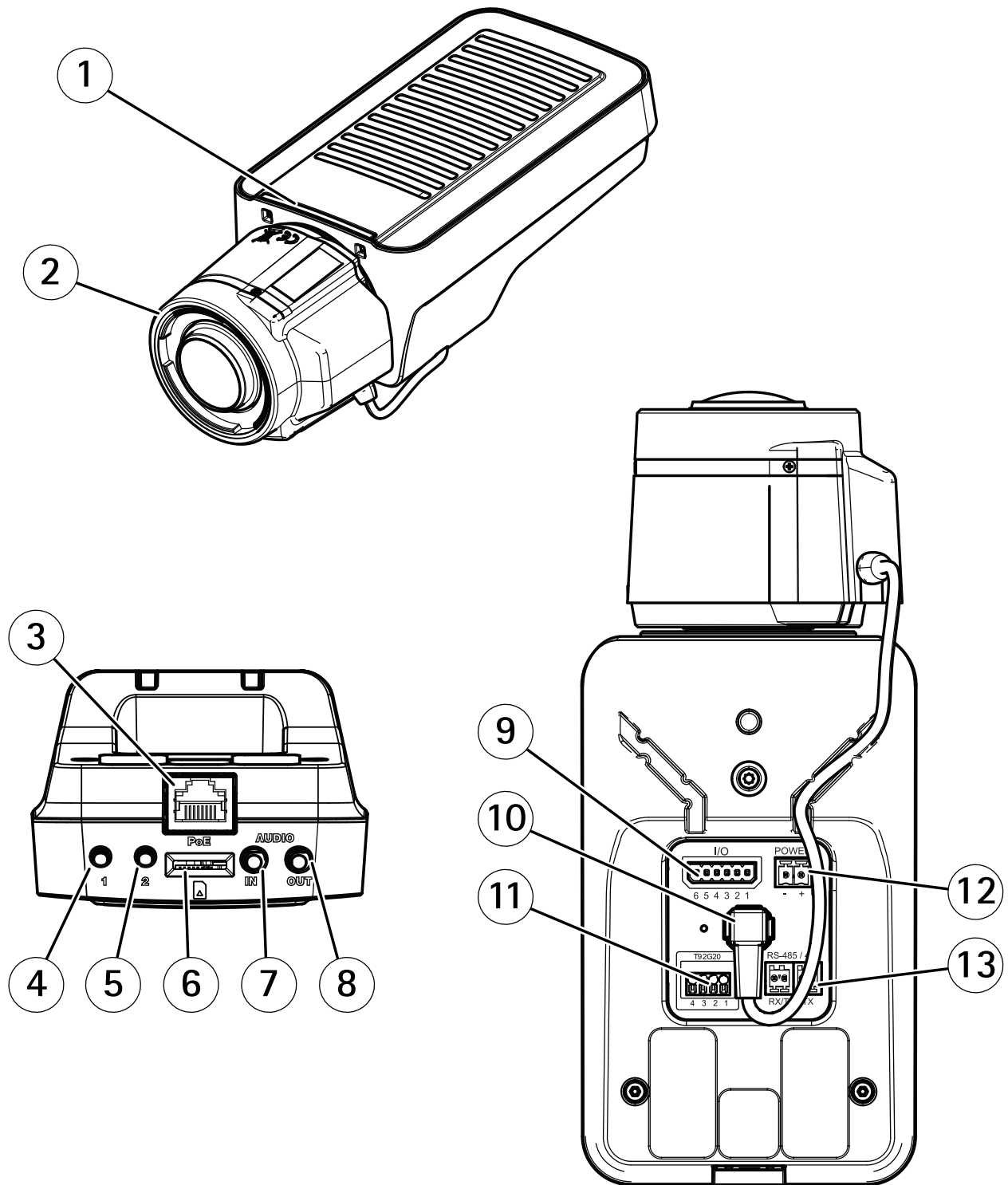
1 Status-LED
