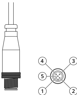
5-pin male A-code DC connector
