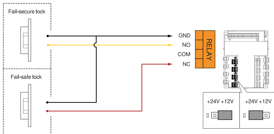
Tür-Relais
